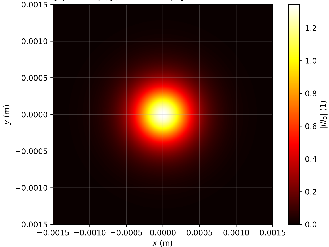
Intensity profile I(x, y, z = 1.274m)/I_0 , Pin=0.8Pcr, artificial time
